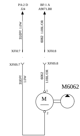
CIRCULATION PUMP, REHEATING SYS
