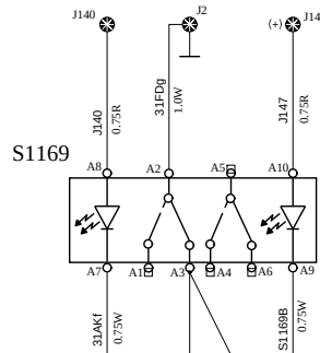
SWITCH, WCL READING LAMPS DASHBOARD
