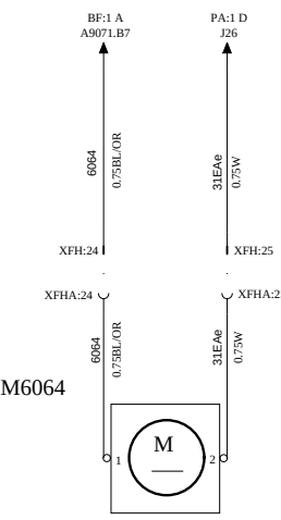
FAN, REHEATING SYSTEM
