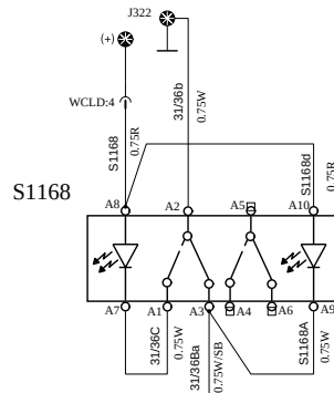
SWITCH, WCL HOST CALL
