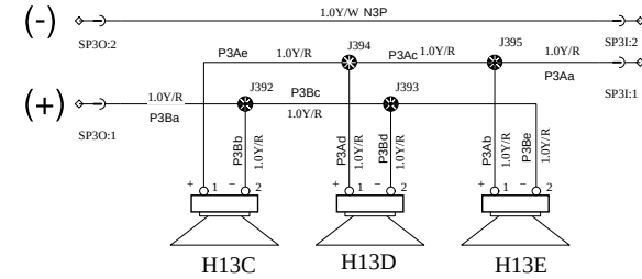
ARRANGEMENT TYPE 2
